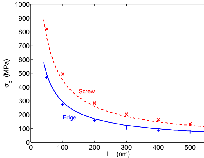
Figure 6. Frank-Read source activation stress for dislocation segments with different lengths in tungsten. Critical stresses predicted by isotropic DD code are plotted as solid and dashed lines for initially edge and screw dislocations, respectively. Critical stresses predicted by anisotropic DD code are plotted as + and × for initially edge and screw dislocations, respectively.
