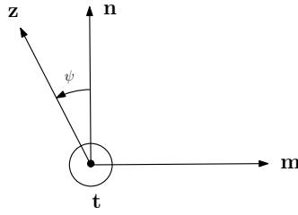
Figure 3. The geometric setup to derive the stress field using the Willis-Steeds-Lothe formula in the collinear case. \mathbf{z} is an arbitrary unit vector in the \mathbf{m} - \mathbf{n} plane at an angle \psi from \mathbf{n} .
