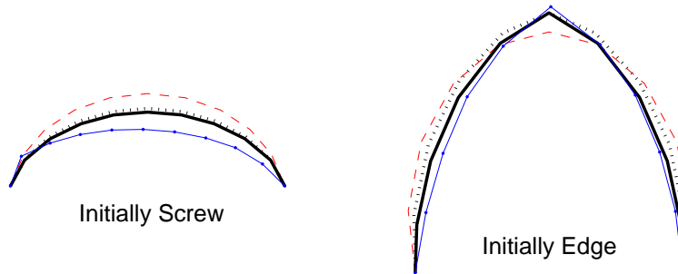
Figure 7. Critical configuration of a Frank-Read source in iron made of an initially screw and an initially edge dislocation segment that is 100-nm long. Anisotropic DD results (thin solid line) is compared with isotropic DD results with different effective elastic constants: Reuss (dotted line), Voigt (dashed line) and Scattergood (thick solid line).
