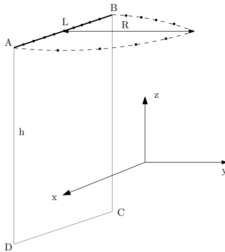
Figure 5. Initial configuration setup used to study Frank-Read source in an isotropic medium.
