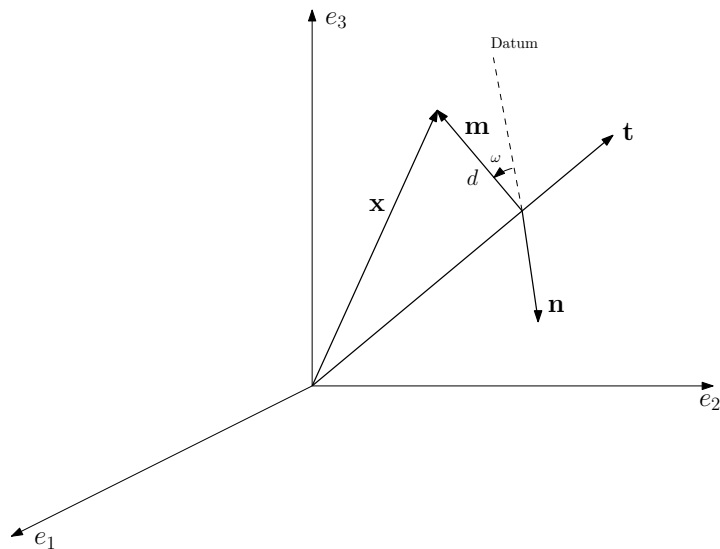
Figure 1. The relationship between \mathbf{m-n-t} coordinate system and \mathbf{e_1-e_2-e_3} crystal coordinate system. The datum is an arbitrary line in the \mathbf{m-n} plane [8].
